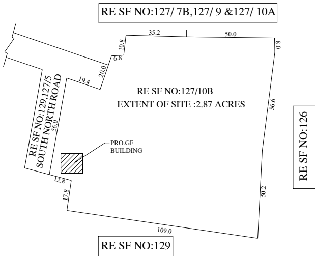
SITE PLAN(NTS)
