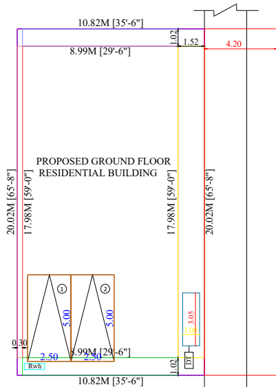
SITE PLAN(MEANT FOR CONSTRUCTION)
