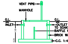
SECTION OF SEPTIC TANK
