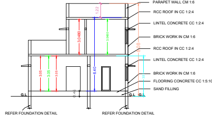
SECTION VIEW 'A-B'
