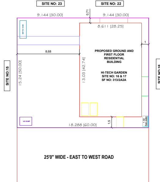
SITE PLAN
