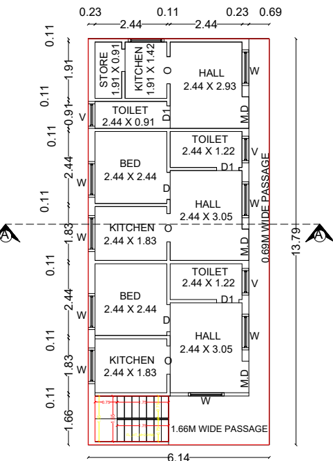
EXI. GROUND FLOOR (G.F) PLAN
