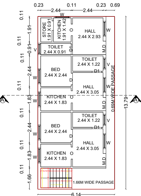
EXI. FIRST FLOOR (F.F) PLAN
