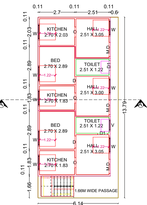
PRO. SECOND FLOOR (S.F) PLAN
