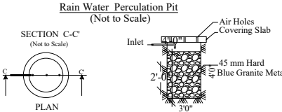
Rain Water Percolation Pit
