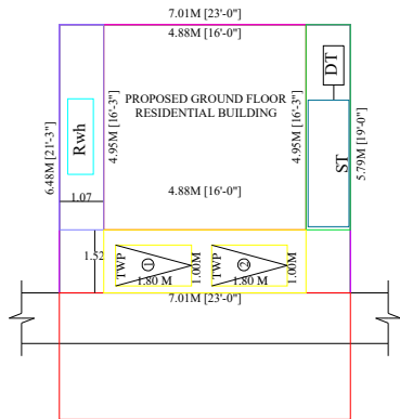
SITE PLAN (MEANT FOR CONSTRUCTION)
