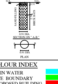
DETAILED PLAN OF RAINWATER PERCOLATION&COLLECTION PIT
