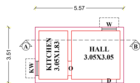
PLAN SCALE 1:100
