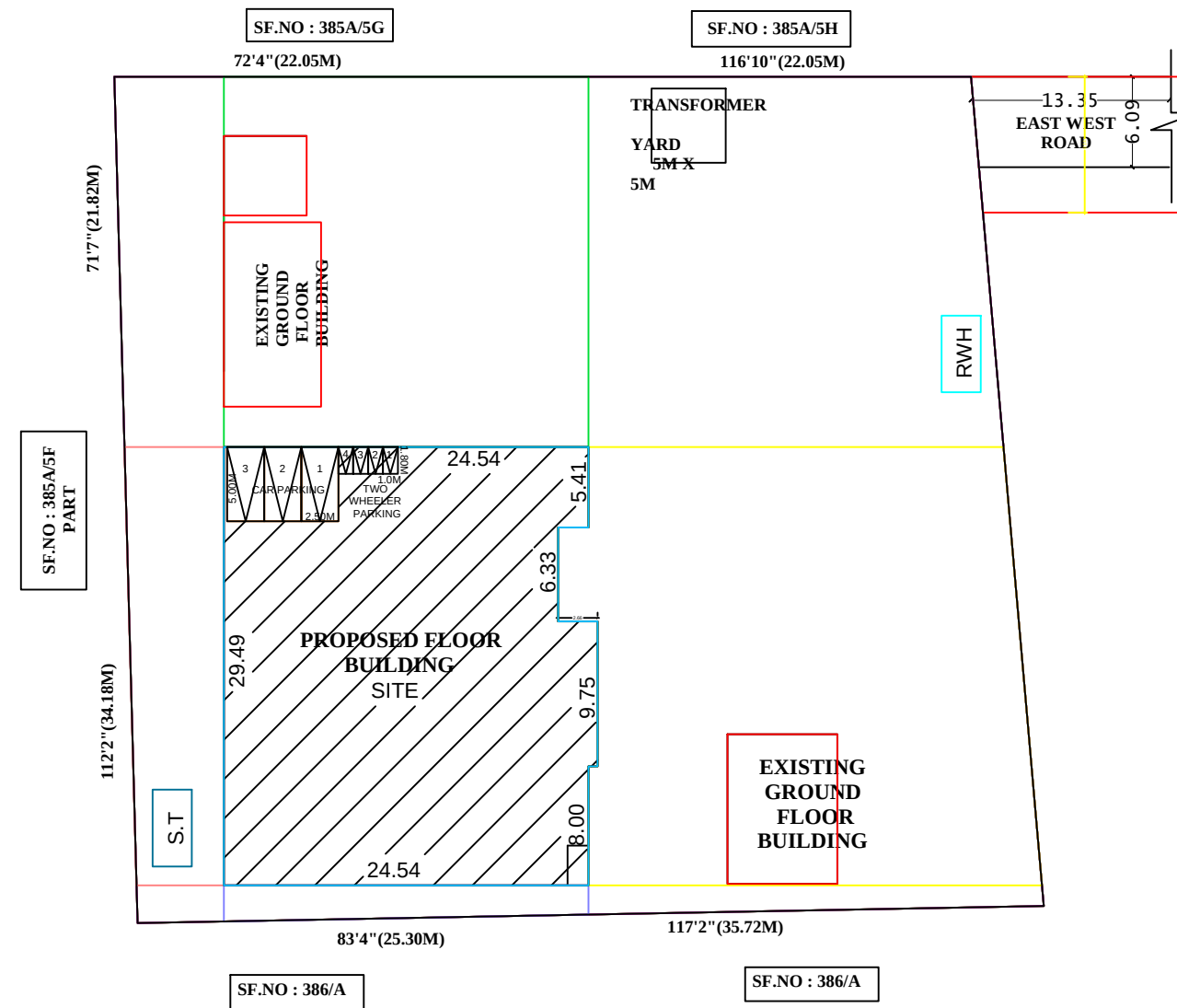
SITE PLAN
