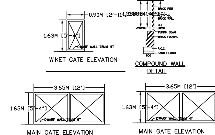
MAIN GATE ELEVATION
