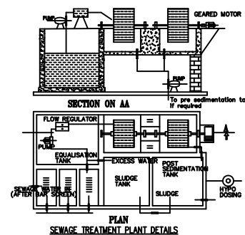
SEWAGE TREATMENT PLANT DETAIL
