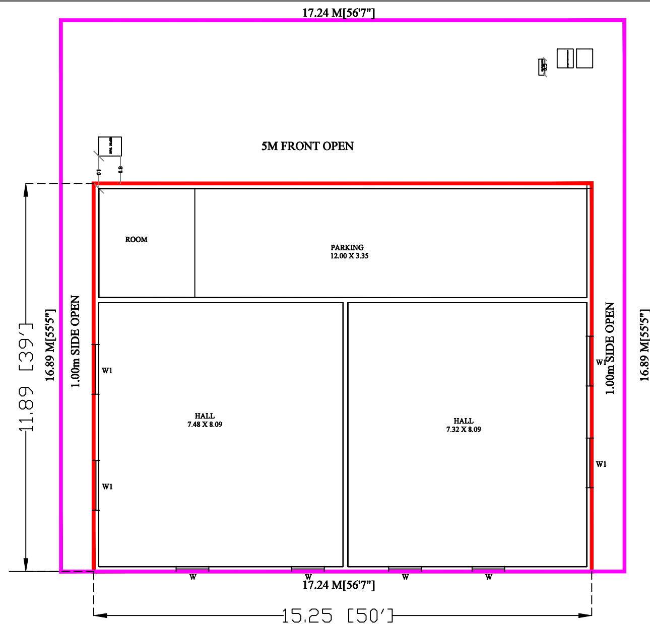
SITE PLAN & GROUND FLOOR PLAN
