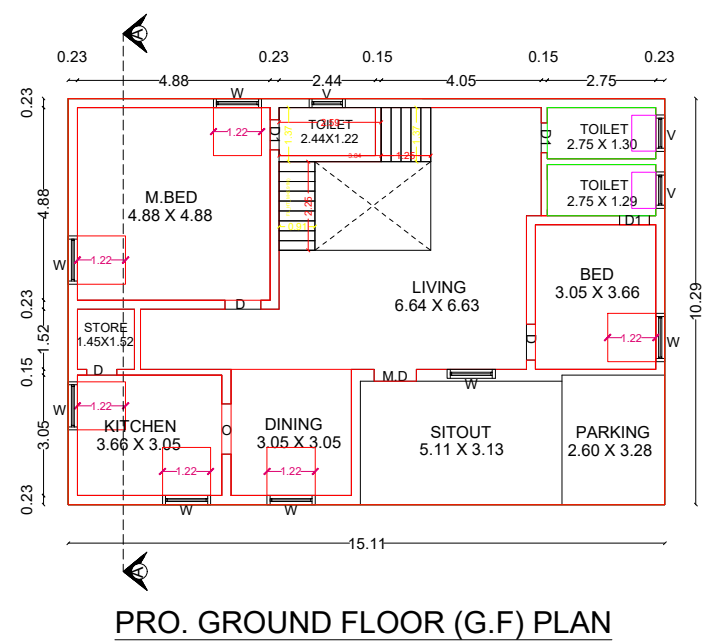
PRO. GROUND FLOOR (G.F) PLAN
