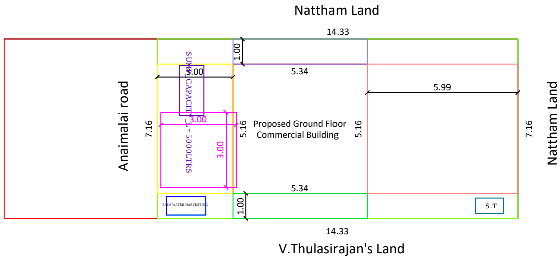
SITE PLAN
