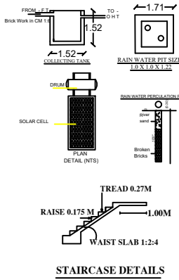
STAIRCASE DETAILS
