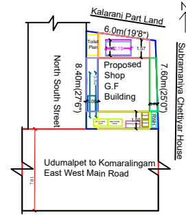
SITE PLAN
