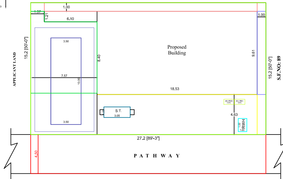
SITE PLAN
