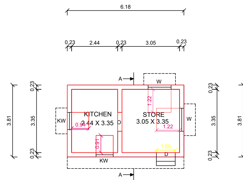
FARM HOUSE PLAN
