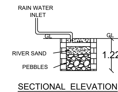
SECTIONAL ELEVATION
