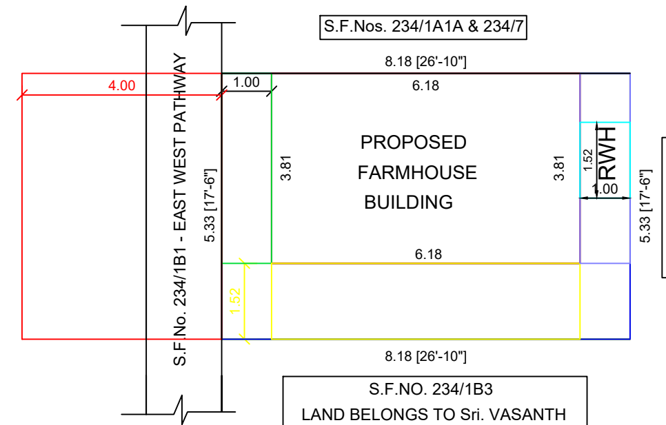
SITE PLAN SCALE : MEANT FOR FARM HOUSE
