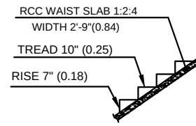
STAIRCASE DETAIL SCALE 1:50
