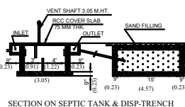
SECTION ON SEPTIC TANK & DISP-TRENCH
