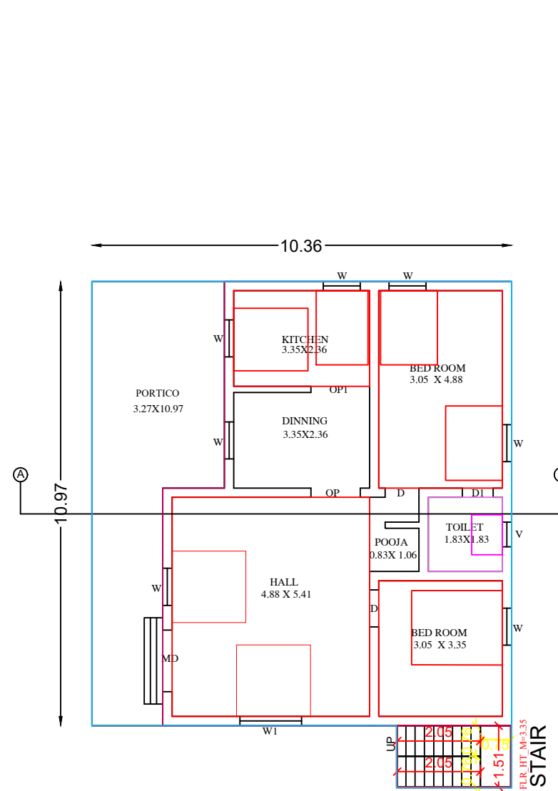
GROUND FLOOR
