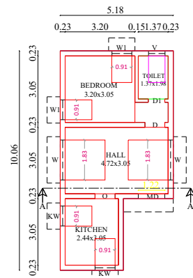
PROPOSED GROUND FLOOR PLAN
