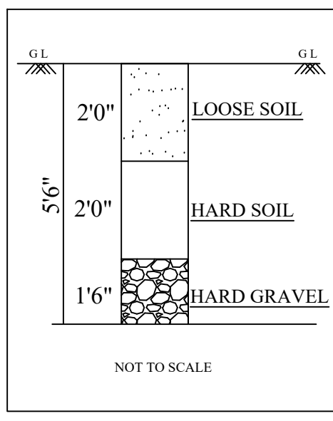
TRIAL PIT
