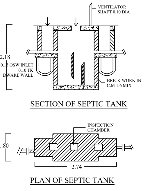
SEPTIC TANK
