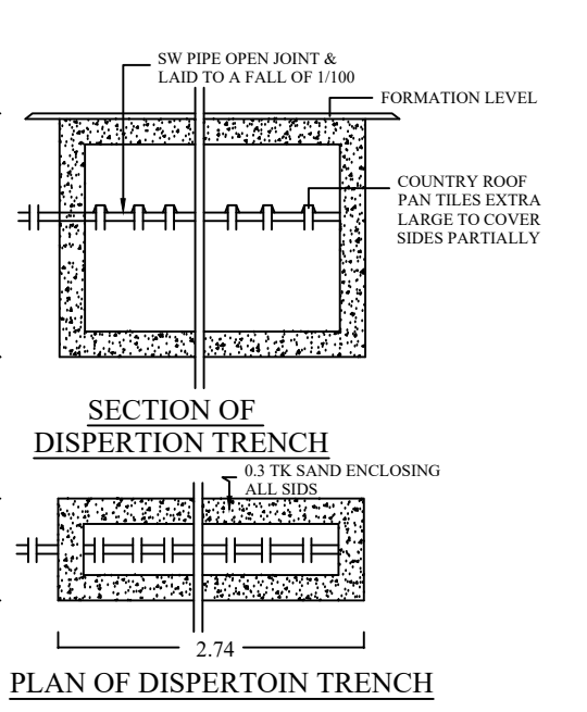
DISPERSION TRENCH
