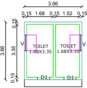
TOILET BLOCK PLAN
