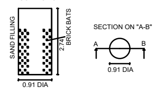
ED PLAN FOR RAINWATER PERCUSSION AND COLLECTION PIT
