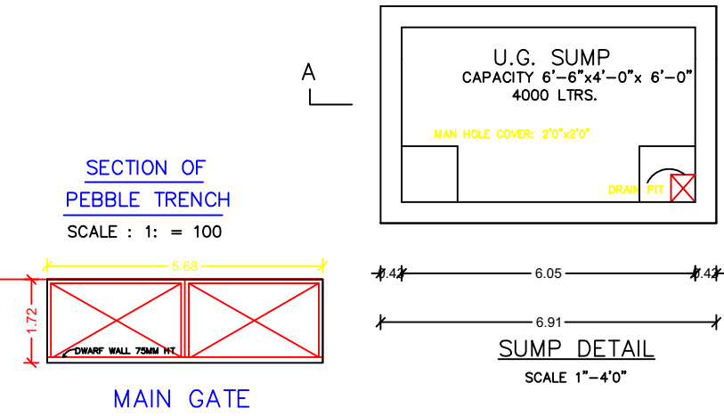
MAIN GATE
