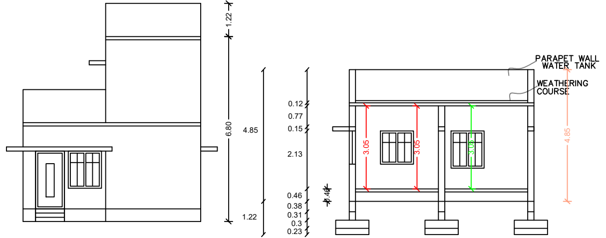
FRONT ELEVATION
