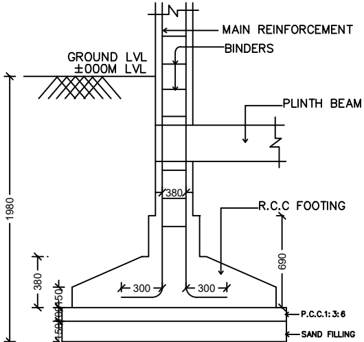
TYPICAL SECTION OF R.C.C. COLUMN FOUNDATION SCALE : 1" = 2'-0"
