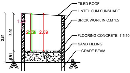
SECTION-AB
