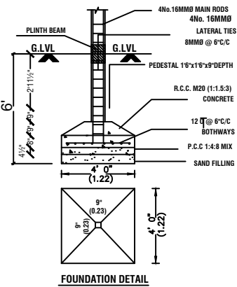
FOUNDATION DETAIL
