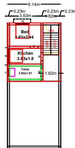
FLOOR - 02
