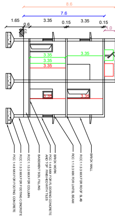
SECTION ON AA
