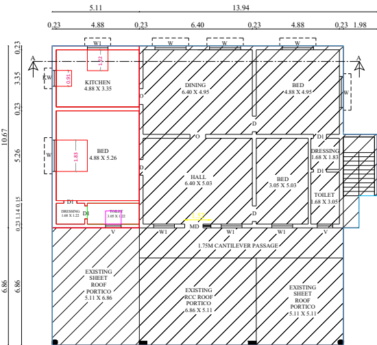
PROPOSED ADDITIONAL CONSTRUCTION WITH EXISTING GROUND FLOOR PLAN
