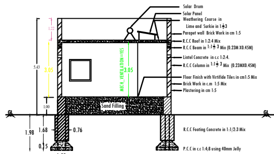
Section on "BC"
