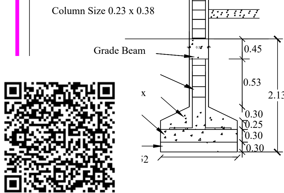
COLUMN DETAILS
