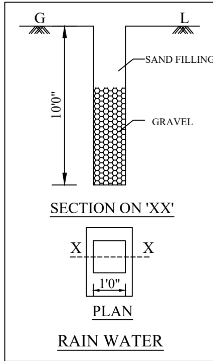
RAINWATER HARVESTING
