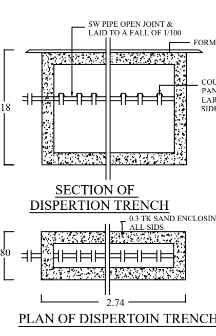
DISPERSION TRENCH
