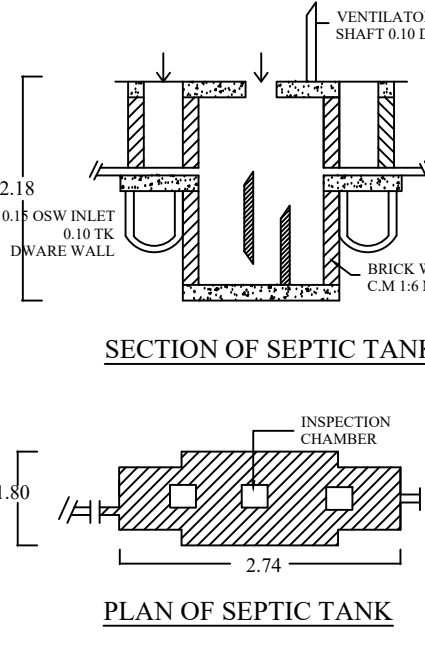
SEPTIC TANK
