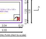
SUMP DETAIL PLAN (Not to scale)
