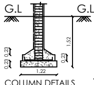
COLUMN DETAILS
