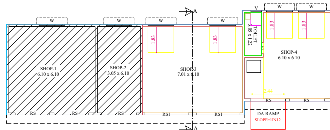
EXISTING ADDITIONAL GROUND FLOOR PLAN
