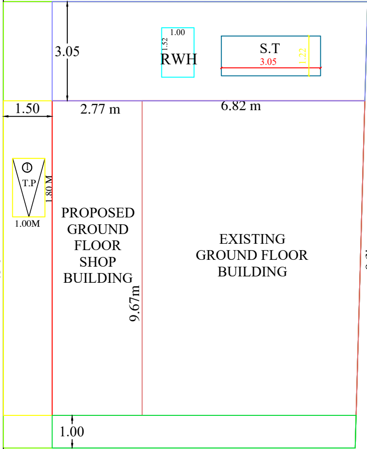
SITE PLAN (1:100)
