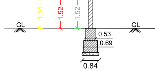
COMPOUND WALL
