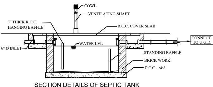
SECTION DETAILS OF SEPTIC TANK
