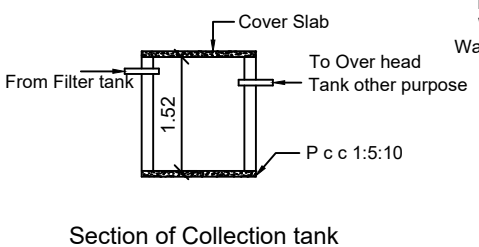
Section of Collection tank
