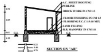
SECTION ON "AB"
