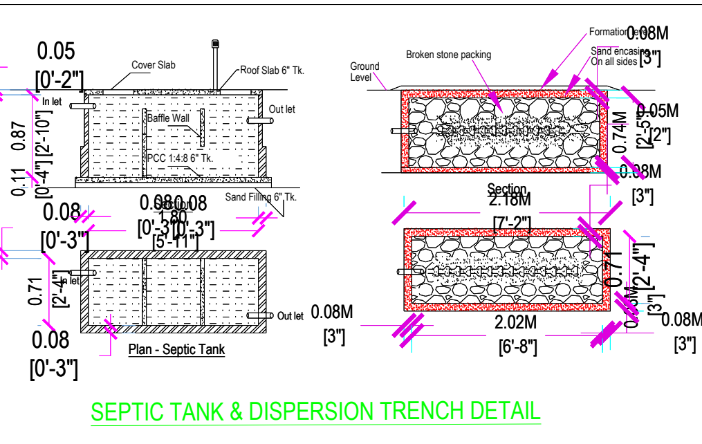
SEPTIC TANK & DISPERSION TRENCH DETAIL
