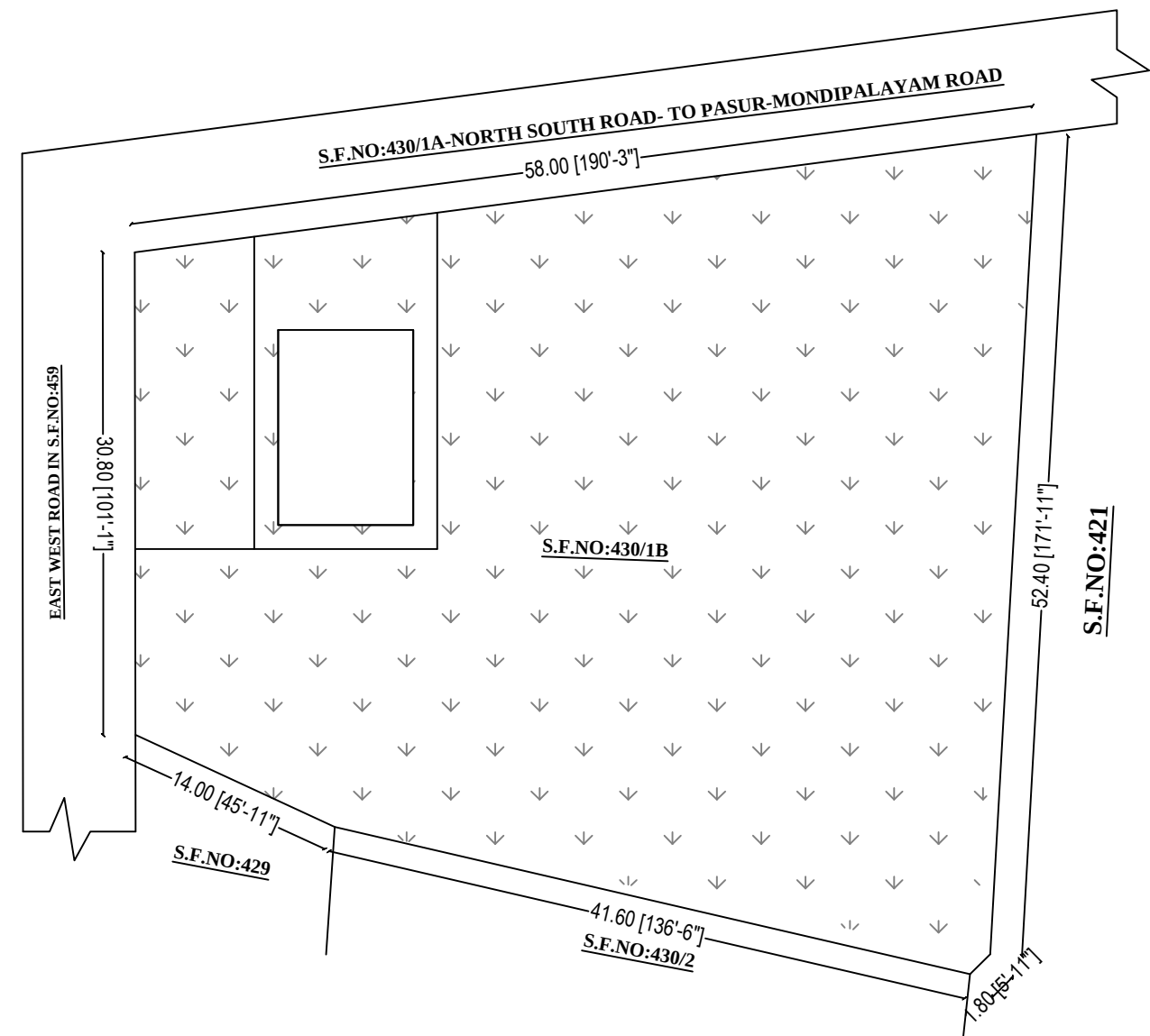
SITE PLAN
