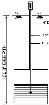
BORE WELL
