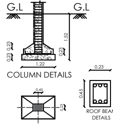
SOLAR POWER PLANT DETAILS
