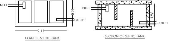
DETAILED DRAWING FOR SEPTIC TANK 225 GALLONS CAPACITY OF 1000 LITRES
