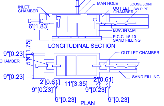
SEPTIC TANK:
