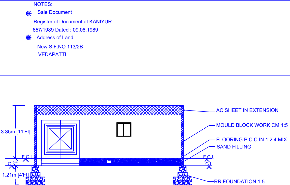
SECTION ON-AA
