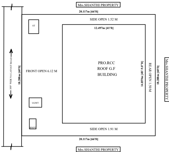
SITE PLAN
