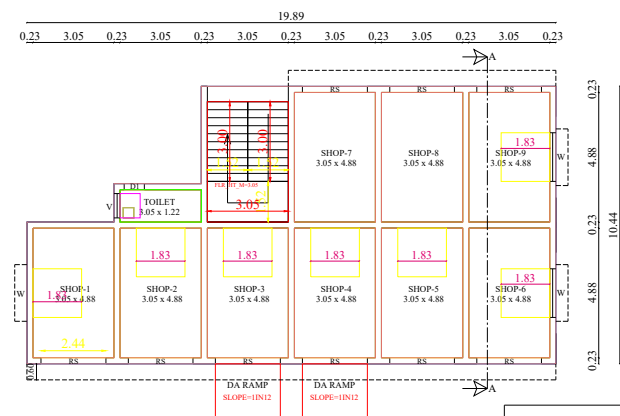
PROPOSED GROUND FLOOR SHOP PLAN
