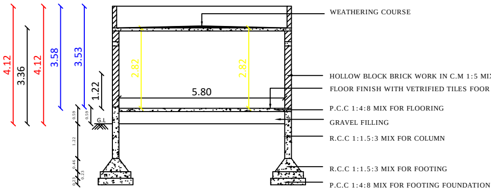
SECTION A-A' (OFFICE)
