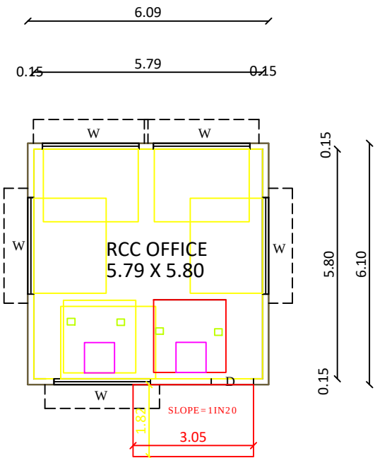
PLAN (BLOCK NO. 1 - R.C.C. OFFICE)
