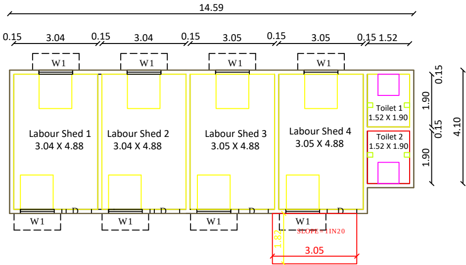
PLAN (BLOCK 2 - A.C. SHEET LABOUR SHED)
