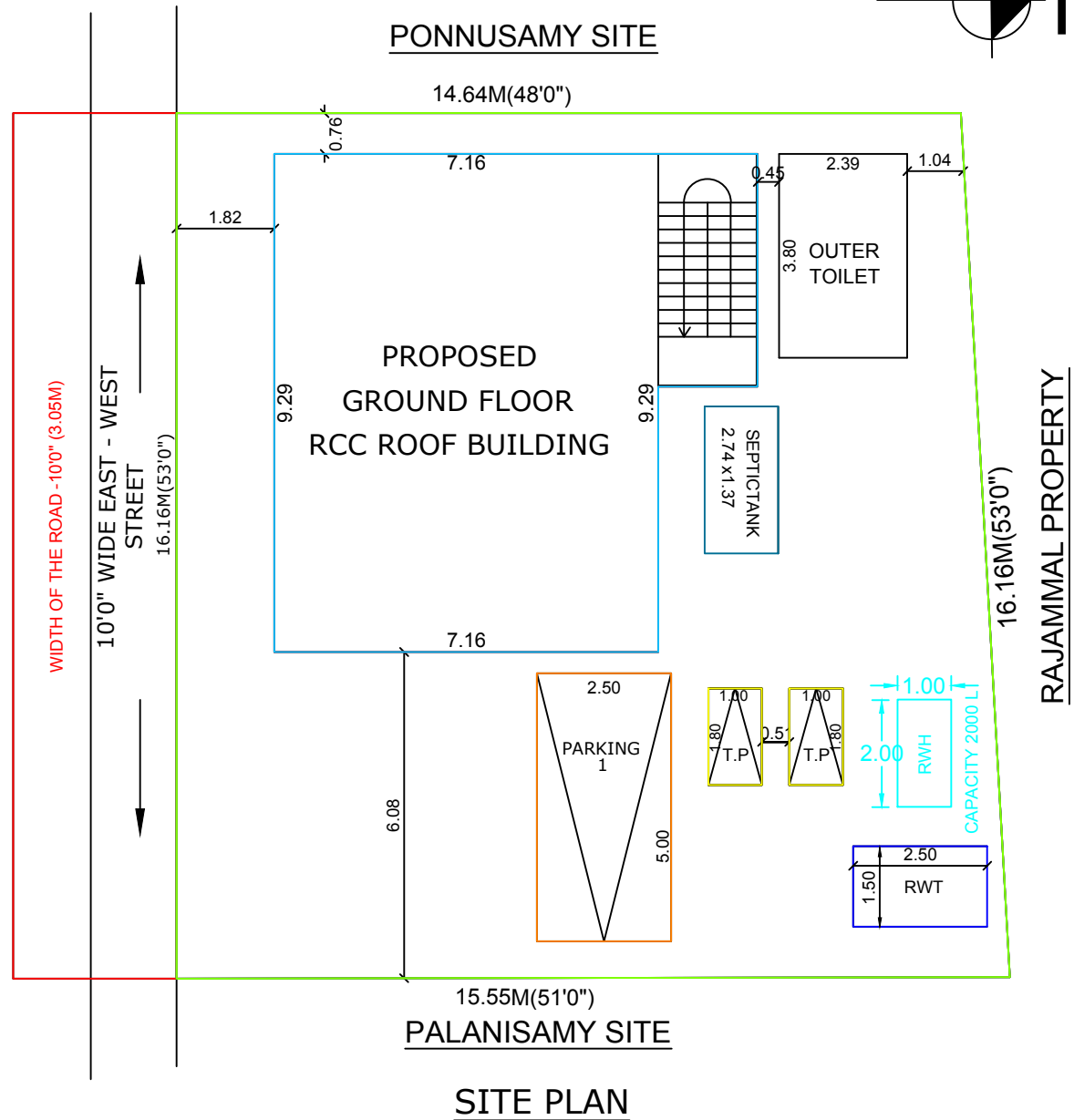
SITE PLAN
