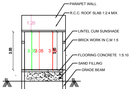
SECTION-AB
