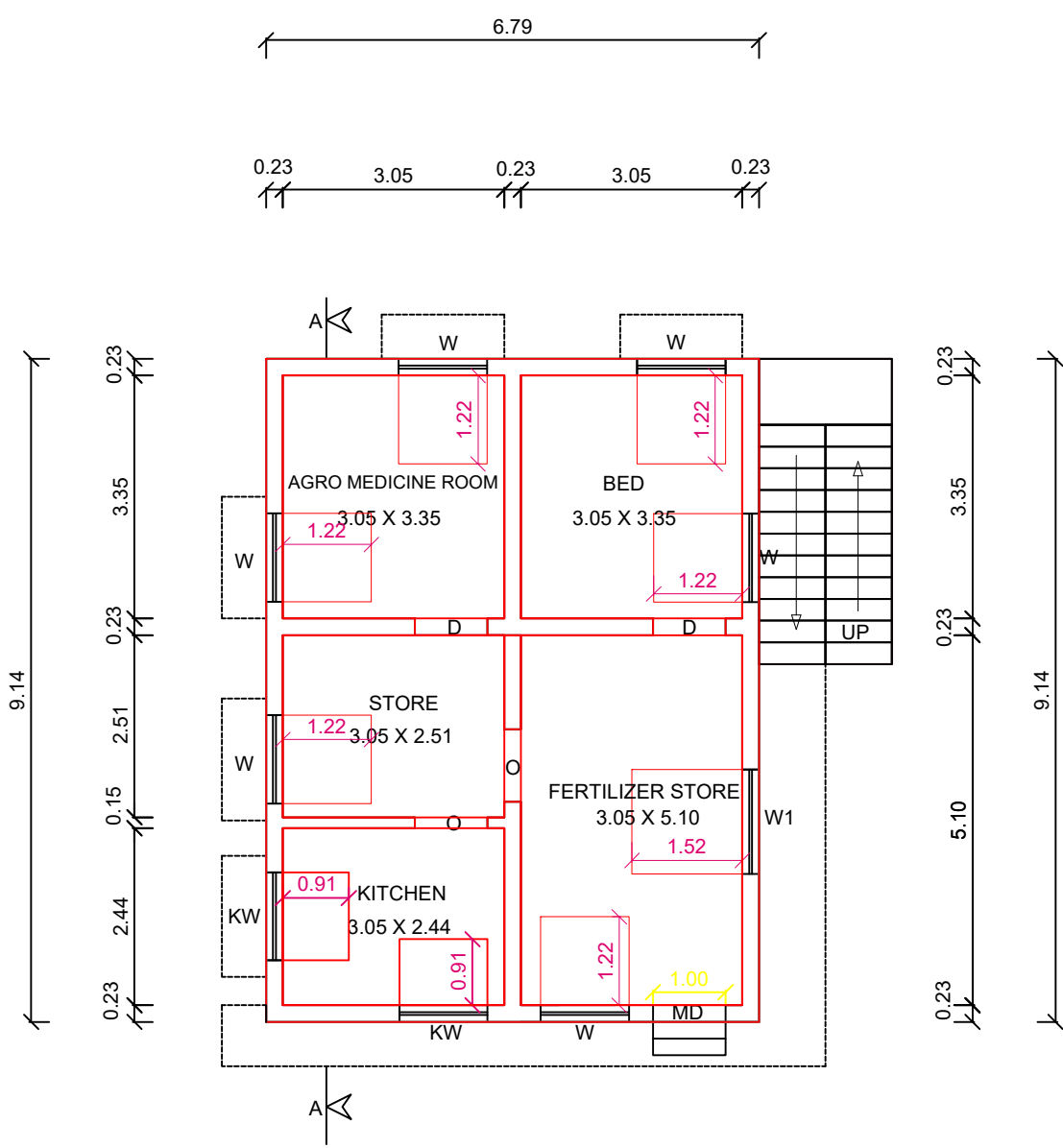
FARM HOUSE PLAN
