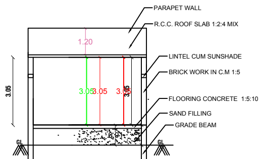
SECTION-AB
