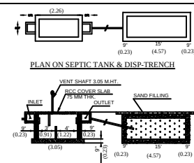
SECTION ON SEPTIC TANK & DISP-TRENCH
