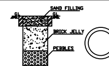
RAIN WATER HARVESTING SYSTEM
