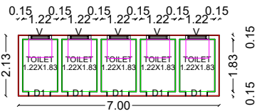
PRO. TOILET PLAN
