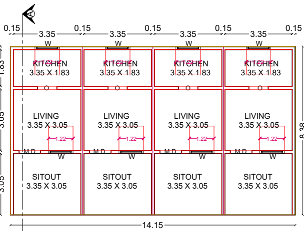
PRO. GROUND FLOOR (G.F) PLAN
