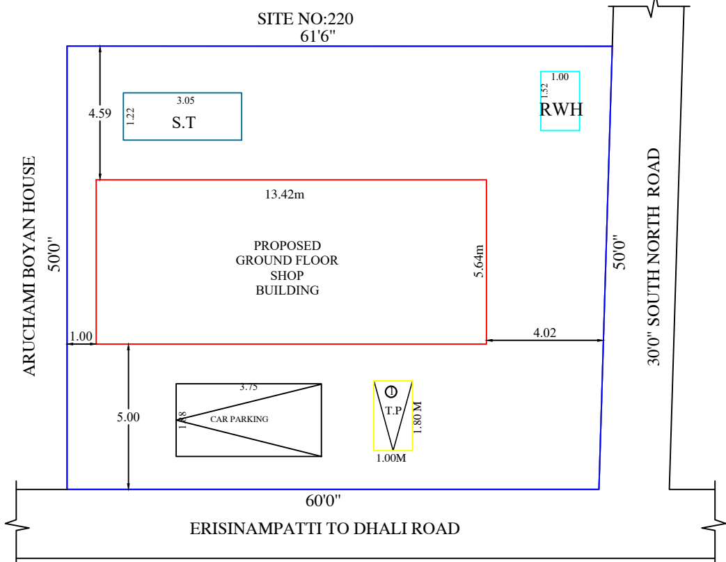
SITE PLAN(1:100)
