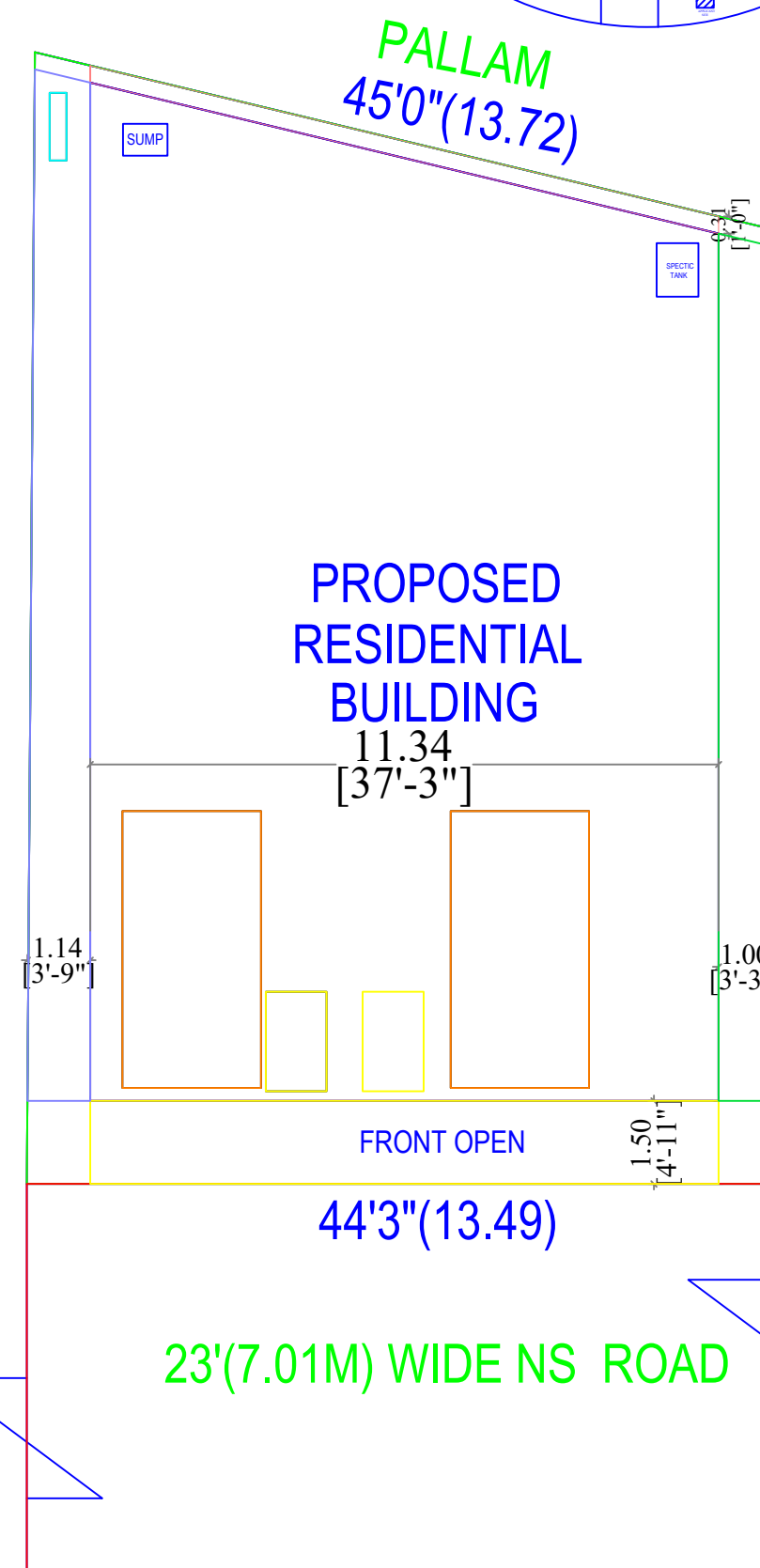
SITE PLAN
