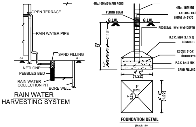
FOUNDATION DETAIL
